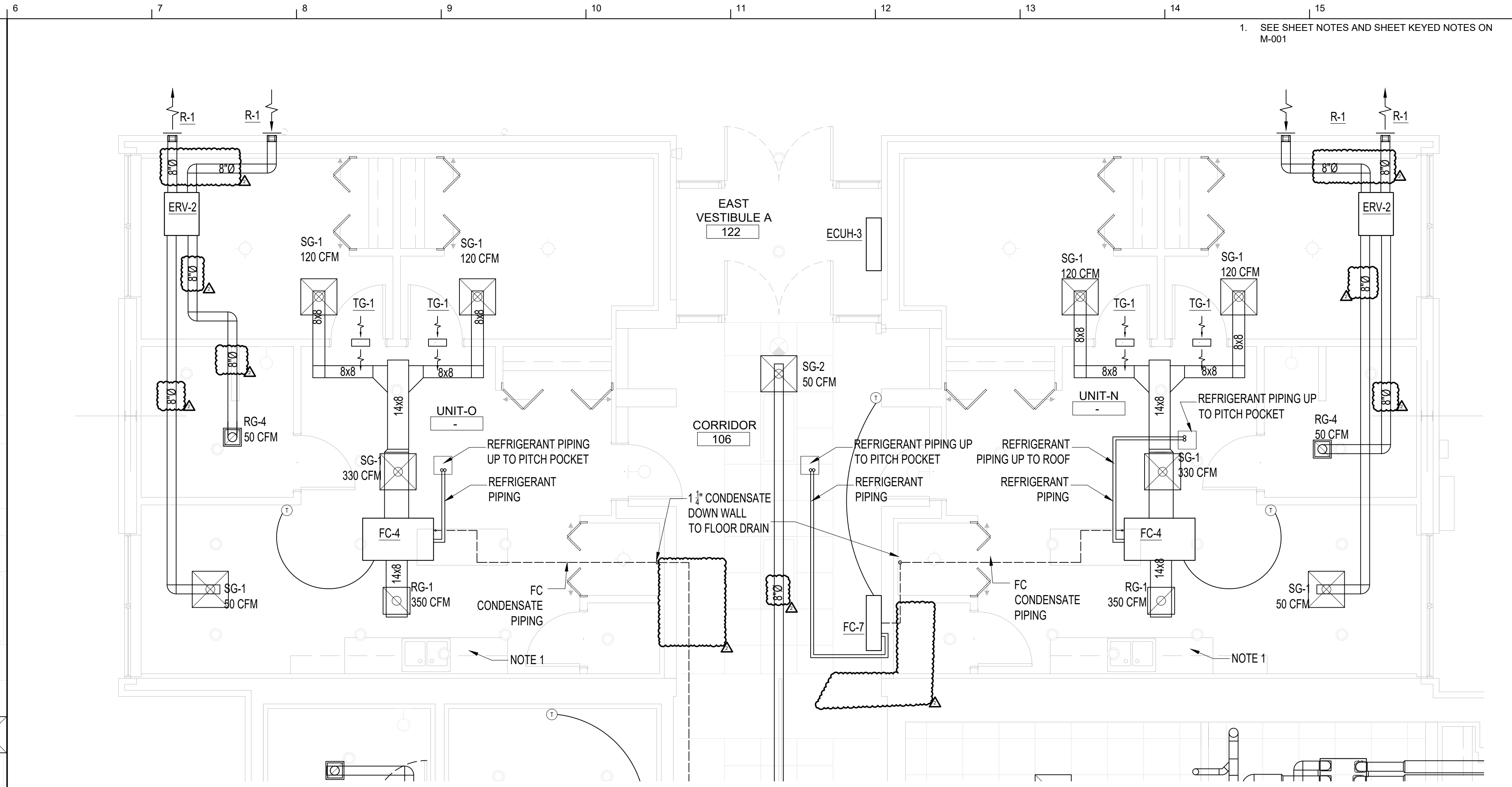
G6 ENLARGED HVAC PLANS
